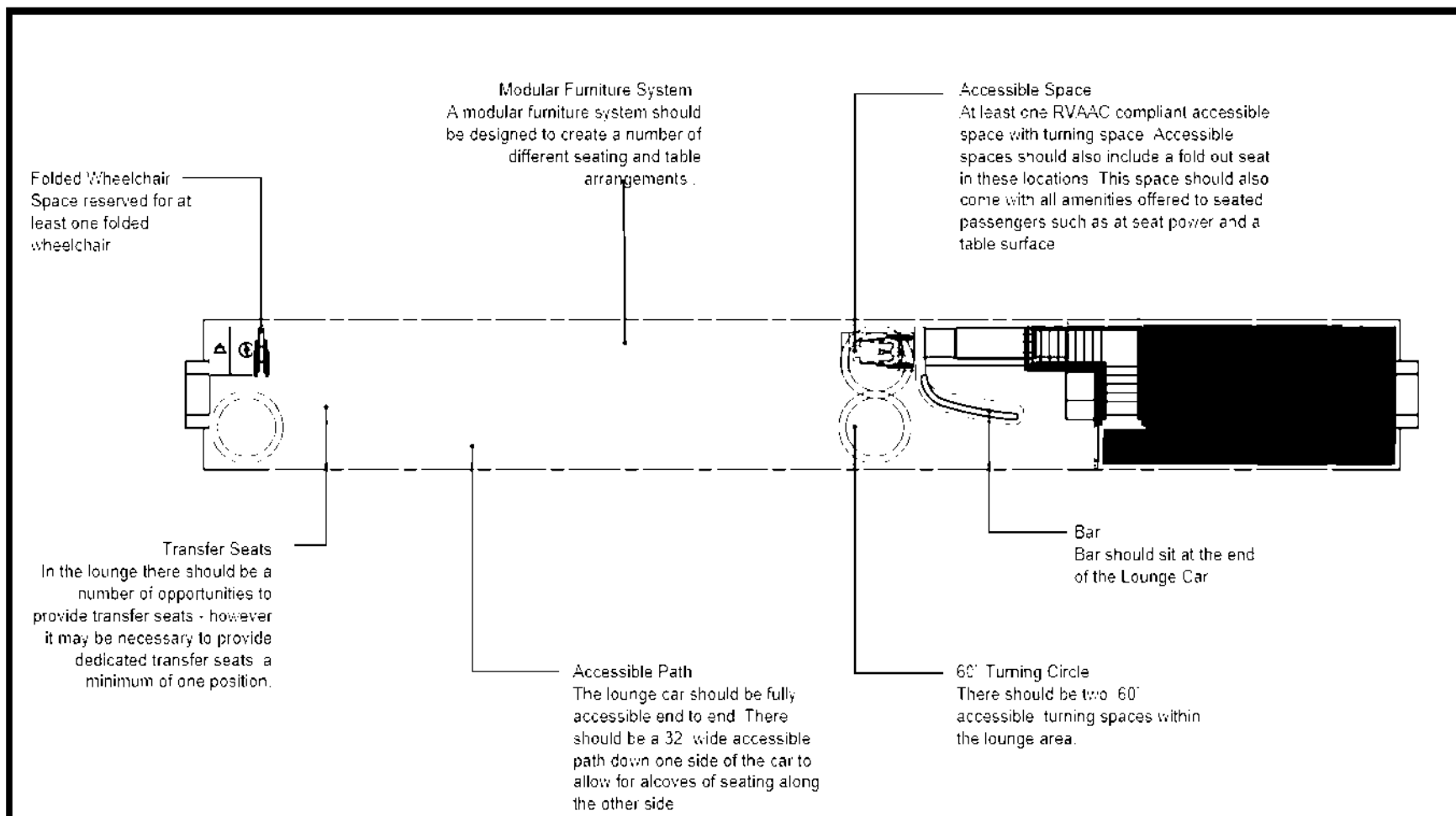
Figure 11-122: Suggested Layout - Lounge
