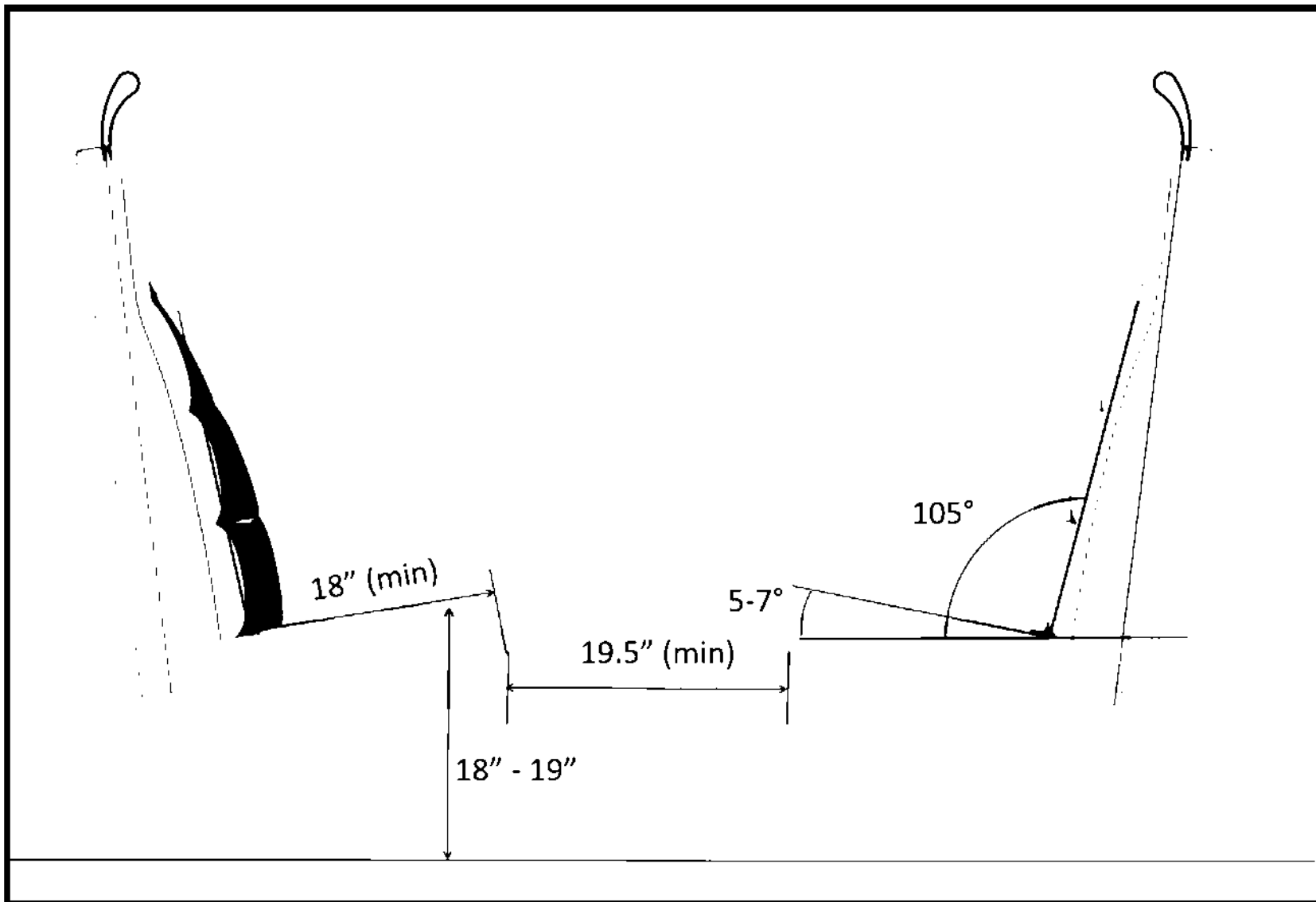
Figure 11-81: Club Bedroom Seat Dimensions
